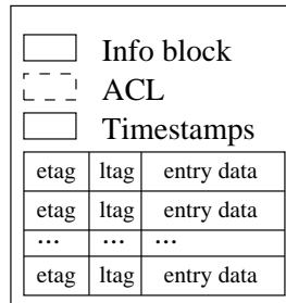
Figure 2.1: The structure of a file object.
