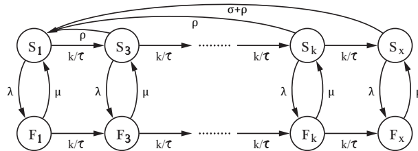
Figure 5: Model of an opportunistically renewed lease.
