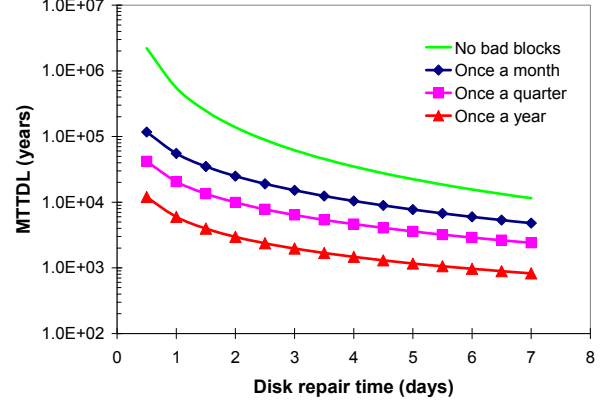
Fig. 2. Expected MTTDL of a RAID level 6 array consisting of ten disks, all subject to disk failures and irrecoverable read errors. Each but the top-most curve corresponds to a specific scrubbing interval.
